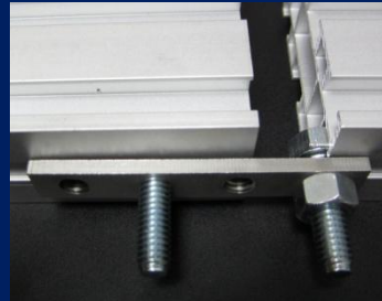
MEPLAT R4 Reinforced flat stainless steel link 15x100 sleek holes.
