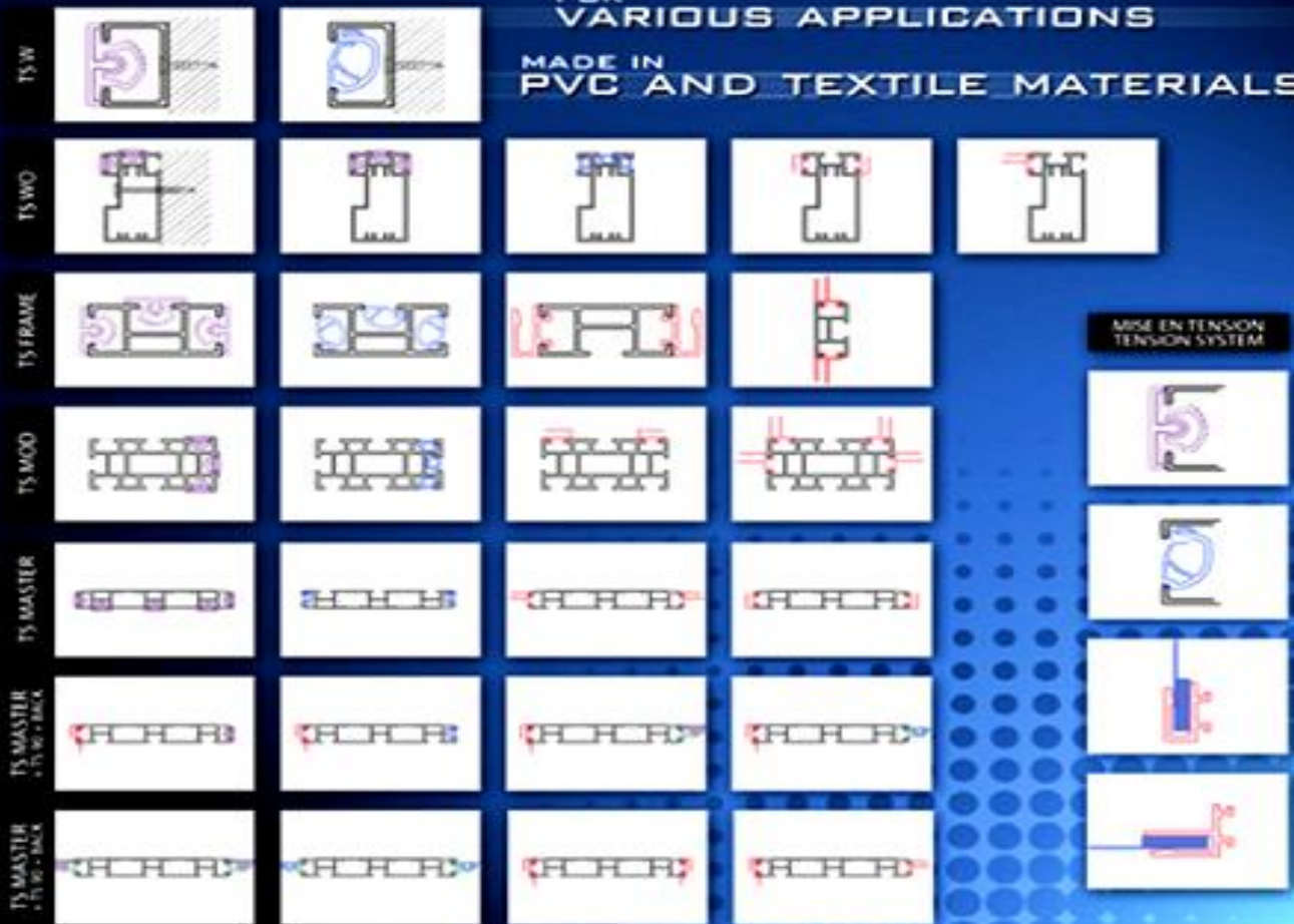
TS90T + Profile For silicone sewn on textile periphery
